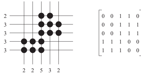
Figure 1: An hv -convex polyomino and the corresponding binary matrix. The elements of the discrete set are marked with black dots. The projections of the polyomino are the vectors H = (2, 3, 3, 3, 3) , V = (2, 2, 5, 3, 2) , D = (0, 2, 3, 2, 1, 1, 2, 2, 1) , and A = (0, 0, 1, 3, 4, 4, 2, 0, 0) .
