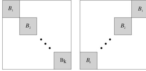
Fig. 4. The relative position of the minimal bounding rectangles of the components B_1, \dots, B_k of a canonical (left) and an anticanonical (right) discrete set.
