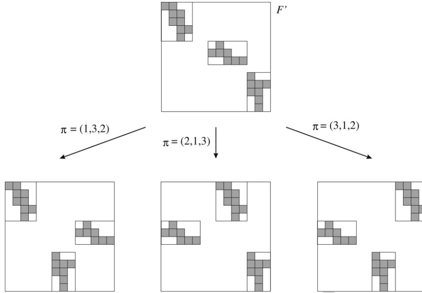
Fig. 5. An example which shows the connection between elements of the \mathcal{H}'\mathcal{V} and \mathcal{S} classes.
