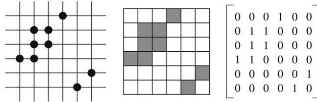
Fig. 1. A discrete set of size 6 \times 6 represented by its elements (left), a binary picture (center), and a binary matrix (right).
