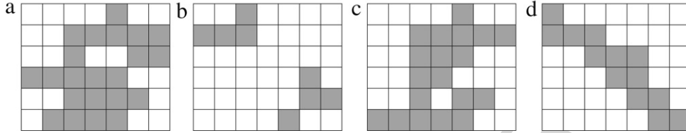
Fig. 2. (a) a polyomino, (b) an hv -convex discrete set, (c) an NE-directed polyomino, and (d) an NW-parallelgram polyomino.
