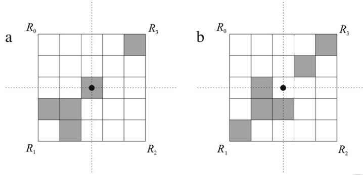
Fig. 3. (a) a Q-convex and (b) a non-Q-convex discrete set with the four quadrants around the point P (denoted by black dot).
