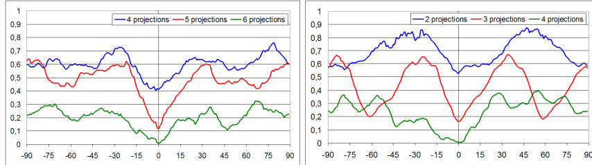
Fig. 5. The graph of RME values after the rotation of the best angle set around the phantoms in Figure 2d (left) and Figure 2e (right) depending on the angle of rotation
