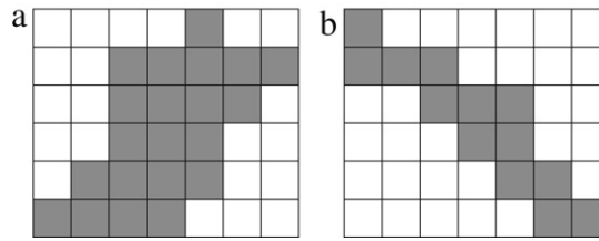
Fig. 3. (a) An hv -convex NE-directed polyomino, and (b) an hv -convex NW-parallellogram polyomino.
