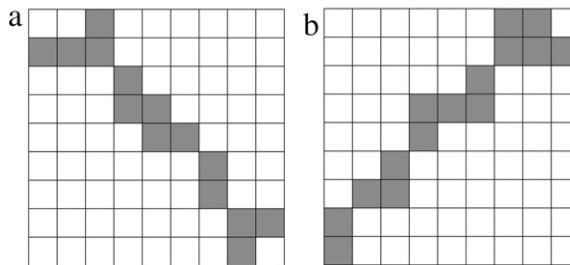
Fig. 4. An hv -convex 8- but not 4-connected set of (a) NW-type and (b) one of NE-type.
