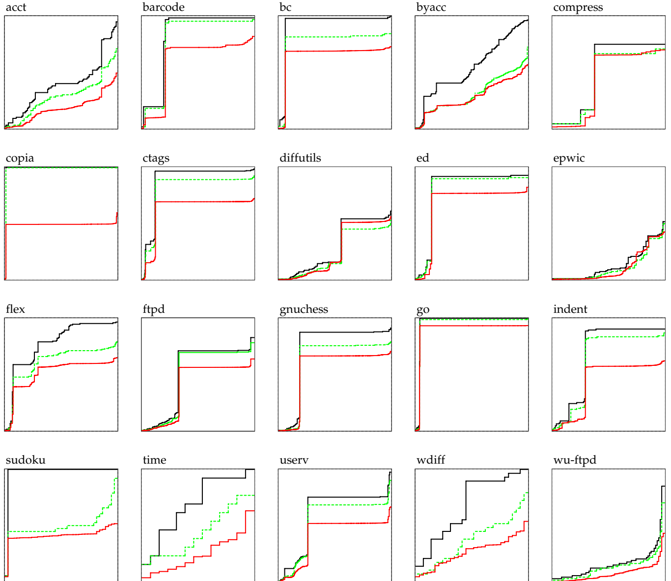
Fig. 1. Subject program MSGs. The lowest solid red line shows Slice^{FV} , the middle dotted green line shows Slice^{FF} , and the upper black line shows Slice^{SEB} . Both axes on the graphs follow the number of program elements (vertices or functions, depending on the slice type) relative to all elements.
