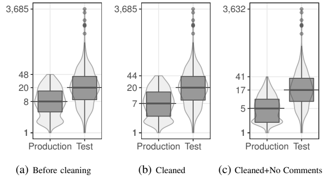
Fig. 3: Distribution of the churn in bug-fixing commits.
