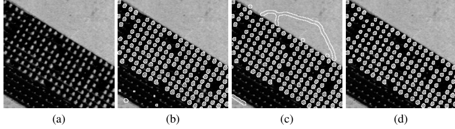
Fig. 2. (a) an image of poplars © IFN (0.6, 0.06, 0.33, 0.19, 2.5); (b) the result with the HOAC ‘gas of circles’ model with inflection point (1160, 0.7); (c) result with the phase field ‘gas of circles’ model (1111, 278, 177.2, 55.8, 30, 4); (d): result with the new model (1160, 0.7, 4).
