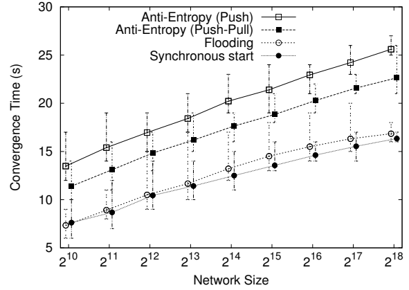
(b) TREE
