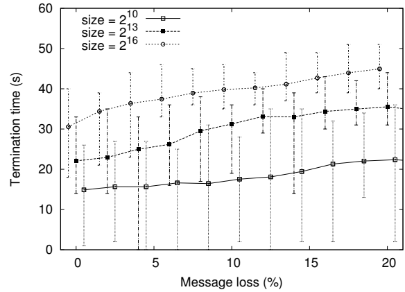
(b) TREE
