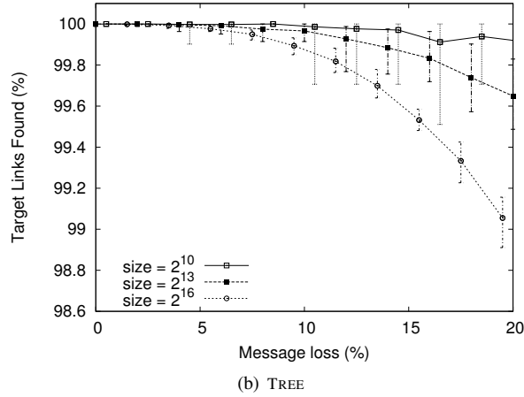
Figure 17: Target links found by the termination time as a function of message loss rate.
