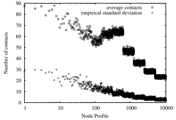
Figure 5: Number of contacts made by nodes while constructing a binary tree. Statistics are over 30 independent runs. The parameters are N = 10000 , m = 20 , number of cycles is 15, \psi = 10 and the tabu list size is 4. In the ranking graph, the root is node 0 and the out-links of node i are 2i + 1 and 2i + 2 .
