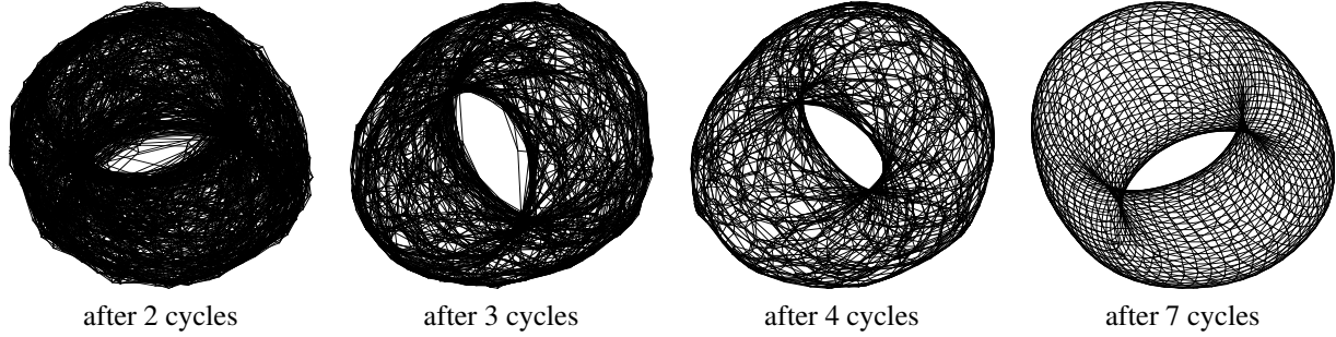
Figure 3: Illustration of constructing a torus over 50 \times 50 = 2500 nodes, starting from a uniform random graph with initial views containing 20 random entries and the parameter values m = 20, \psi = 10, K = 4 .
