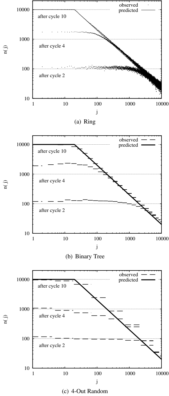
Figure 8: Experimental and predicted values of n(j) for three different ranking graphs. Experiments were run with N = 10000 , m = 20 and \psi = 10 , without a tabu list. Note that the plots contain three snapshots of the simulation for cycles 2, 4 and 10. In Figure (a), the dots representing the situation after 10 cycles for values j \leq 100 are covered by the predicted line.
