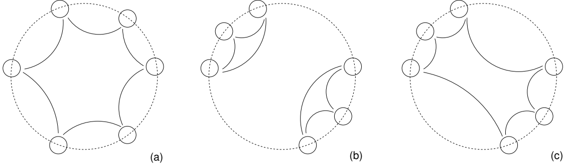
Figure 1: Target graphs for different ranking methods and K = 2 . (a) One-dimensional distance-based, circular ranking method applied to a set of uniform node profiles; (b) same ranking method as before but with a different set of node profiles that are clustered; (c) direction-dependent ranking method achieves sorting even for clustered node profiles.
