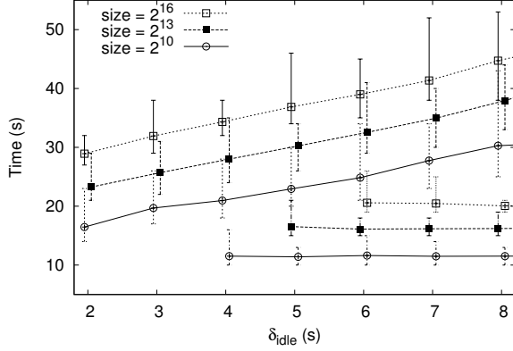
(b) TREE
