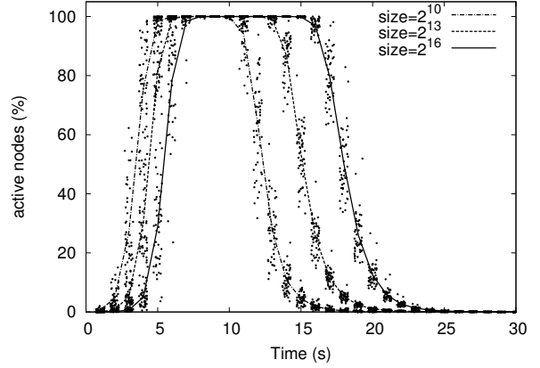
(b) TREE
