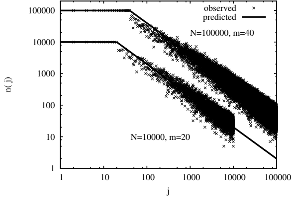
Figure 7: Experimental results and values predicted by Equation (2) for n(j) with two sets of parameters N = 10000, m = 20 and N = 100000, m = 40 . For each j , the converged value of n(j) is indicated as a separate point. The observed values correspond exactly to the predicted one for the initial constant section, and are covered by the line segment on the graph.
