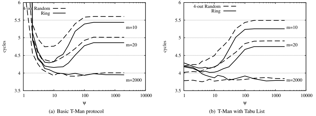
Figure 4: Time to collect 50% of the neighbors at distance one in the ranking graph. Network size is N = 2000 . Node views are initialized to contain 5 random links each. Graph (b) was obtained using a tabu list of size 4.
