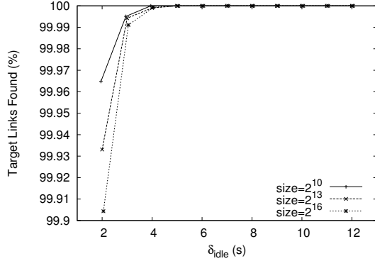
Figure 12: Quality of the target TREE graph at termination time as a function of \delta_{idle}
