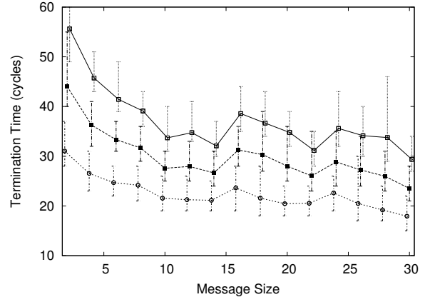
(b) TREE
