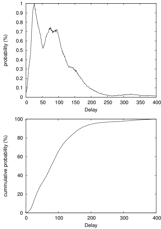
Figure 9: Probability distribution of end-to-end delays as reported in the King data set [28].
