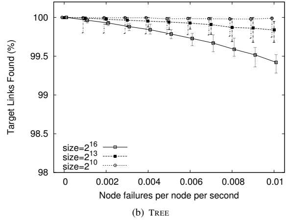
Figure 18: Target links found by the termination time as a function of failure rate.
