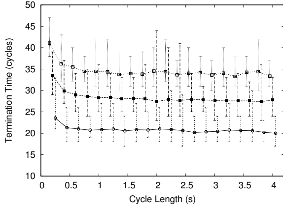
(b) TREE
