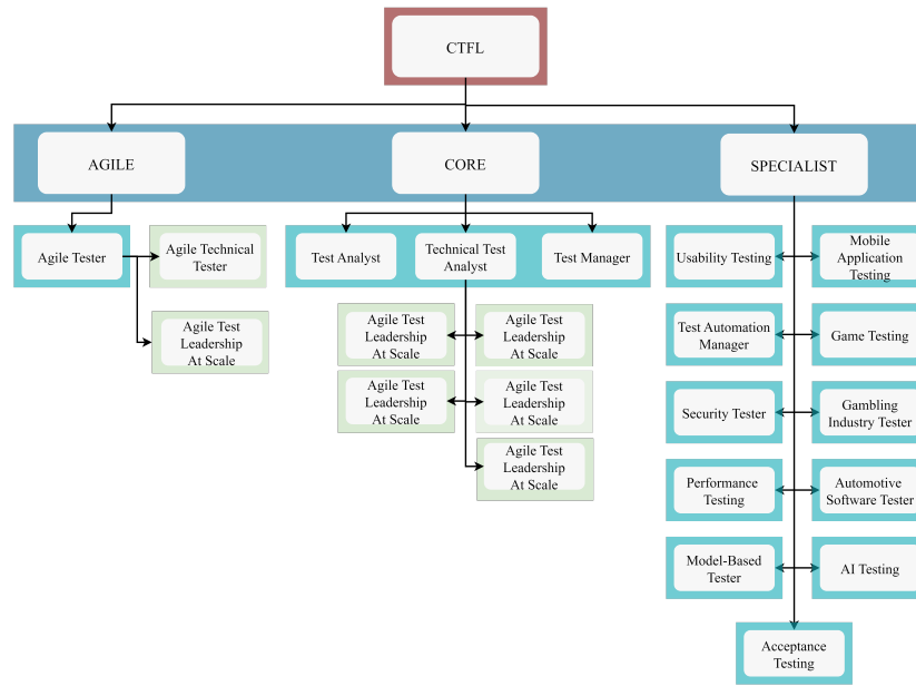
Fig. 1. ISTQB certifications
