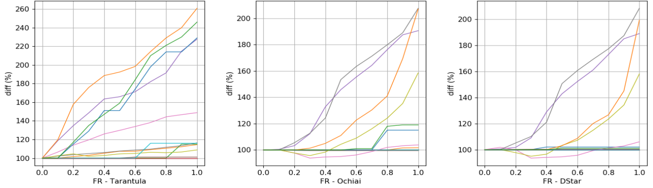
Fig. 4: Results – more failed tests (one line represents the results for one bug)
