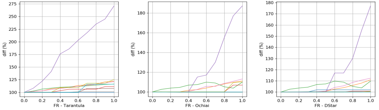
Fig. 6: Results – more faulty methods (one line represents the results for one bug)
