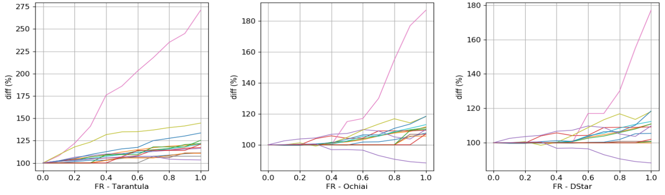
Fig. 3: Results – one failed test (one line represents the results for one bug)
