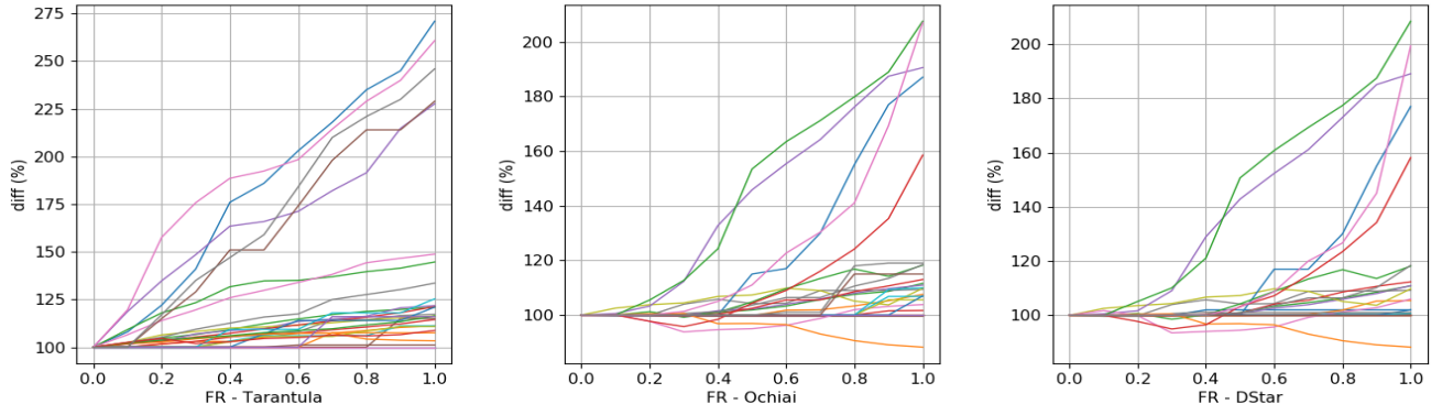
Fig. 1: Tarantula, Ochiai and DStar results (one line represents the results for one bug)
