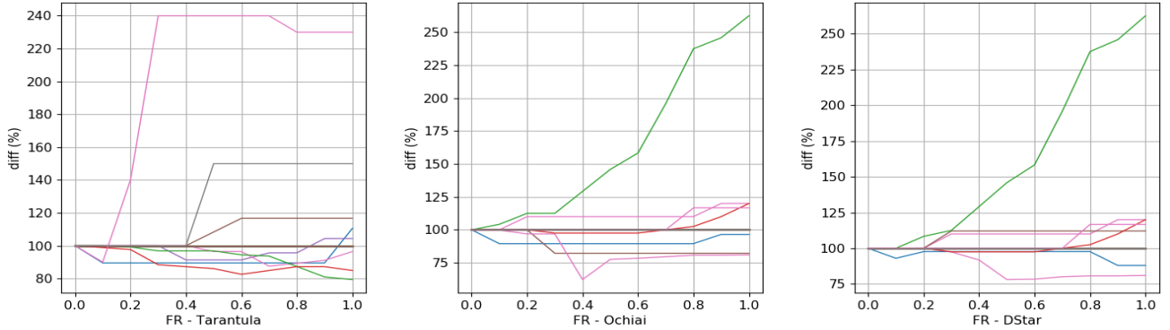
Fig. 7: Tarantula, Ochiai and DStar – failed tests (one line represents the results for one bug)
