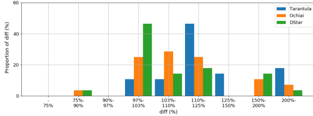
Fig. 2: Tarantula, Ochiai and DStar diff - FR:1.0
