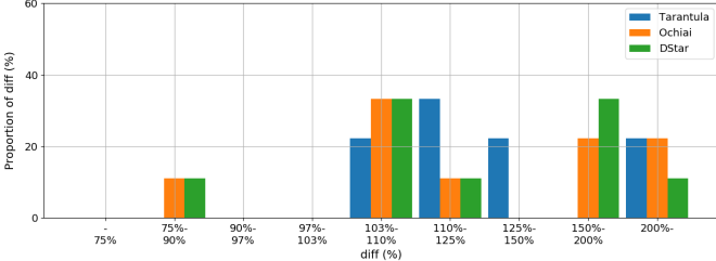
Fig. 10: Tarantula, Ochiai and DStar – high \phi_{ep}
