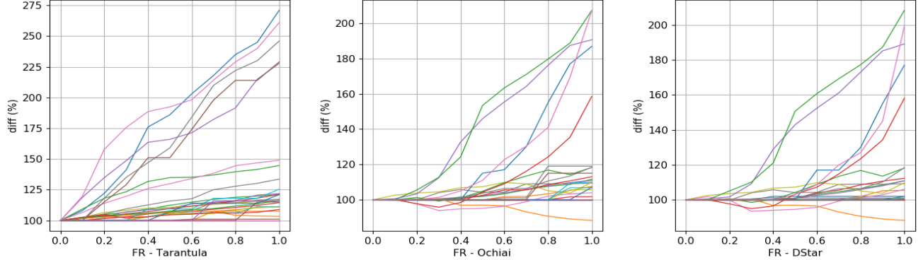
Fig. 8: Tarantula, Ochiai and DStar – passed tests (one line represents the results for one bug)
