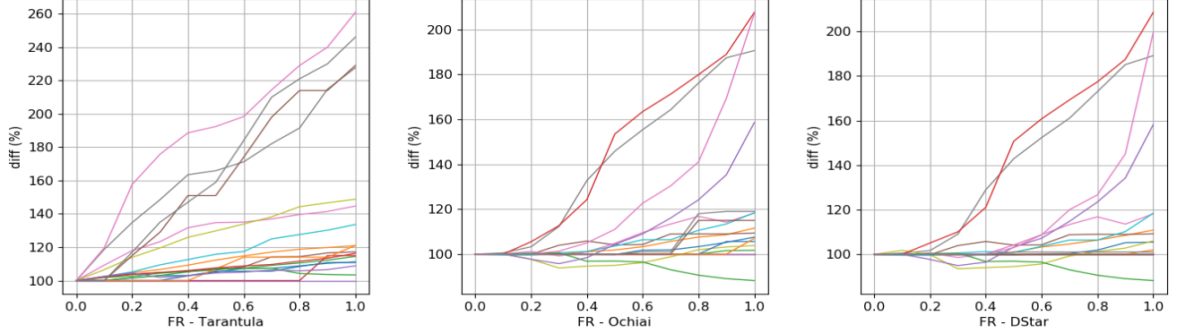
Fig. 5: Results – one faulty method (one line represents the results for one bug)
