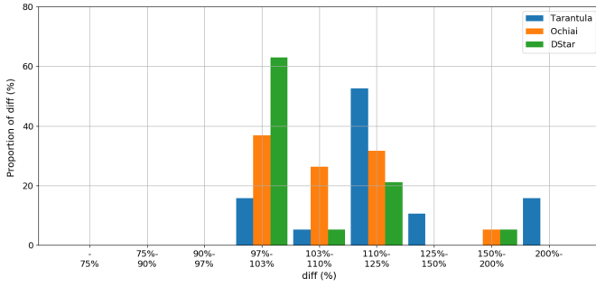
Fig. 9: Tarantula, Ochiai and DStar – low \phi_{ep}
