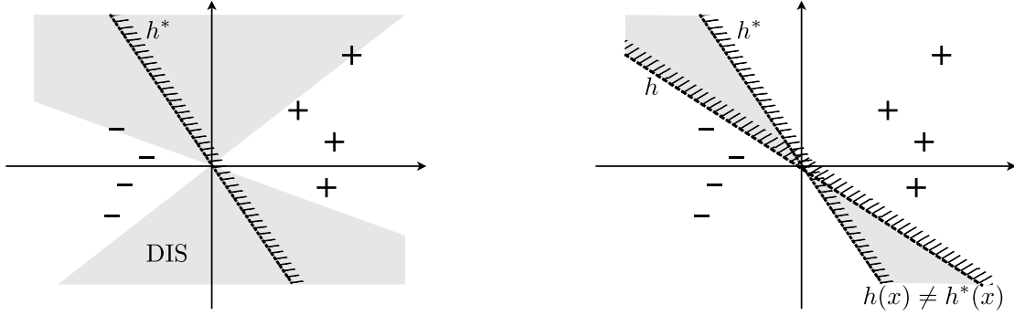
Figure 1: An illustration of the disagreement region. Let X be \mathbb{R}^2 and let \mathcal{C} be the class of homogenous half planes. The target concept h^* is denoted by the dashed line and the positive and negative sample points in X' are given by “+” and “-”. The gray area represents the resulting disagreement region in the first picture and the error region of the consistent hypothesis h in the second. Please note that the largest possible error can never cover the whole disagreement region, and therefore \theta(\mathcal{C}) > 1 .
