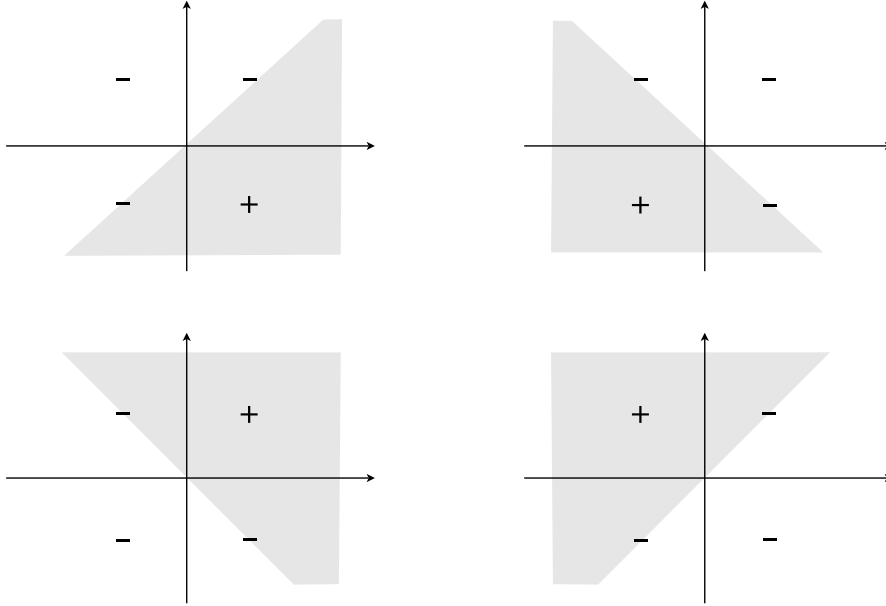
Figure 4: Using four fixed points, one can find the singletons of size four as a subclass of the open, homogenous half planes. A co-singleton class of size four is induced by the complementary, closed half planes.
