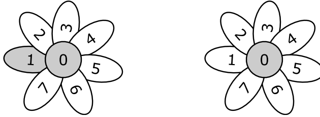
Figure 2: The drawing depicts the concepts \{0, 1\} and \{0\} in \text{SF}_7 . Each concept in \text{SF}_n consists of the kernel 0 and at most one of the petals 1, \dots, n . The class is named after the sunflower and fulfills the well known definition of “sunflower” in combinatorics, but is otherwise unrelated.
